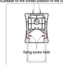
TYPE A : Screw fixing position
